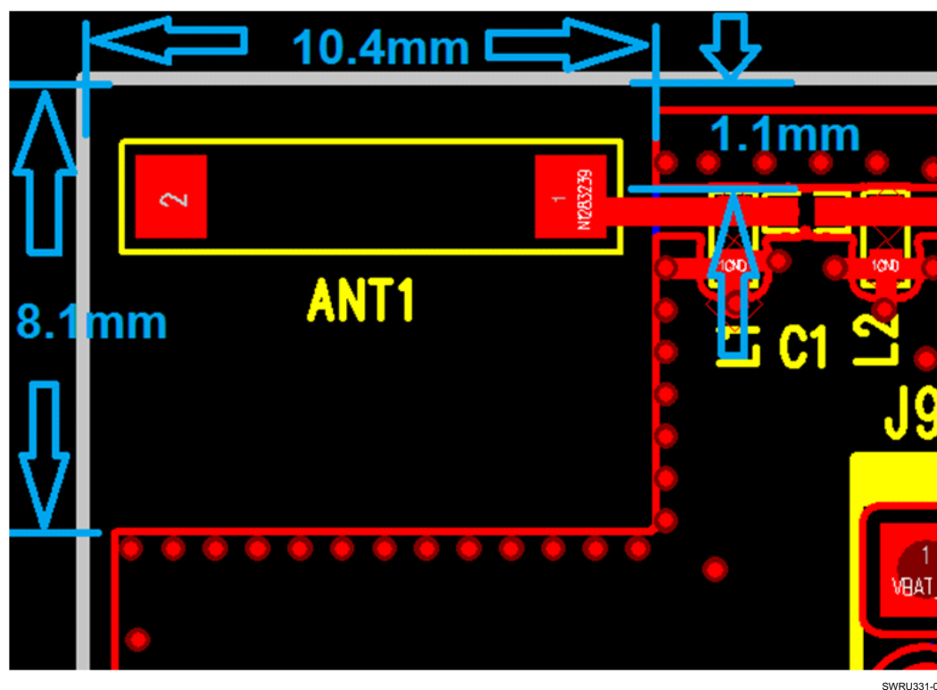
Figure 2-10. Antenna Layout Guidelines
